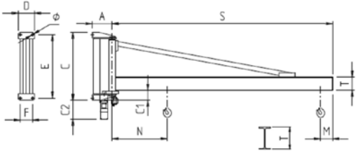
290° Wall-mounted jib crane Rotation 290°
