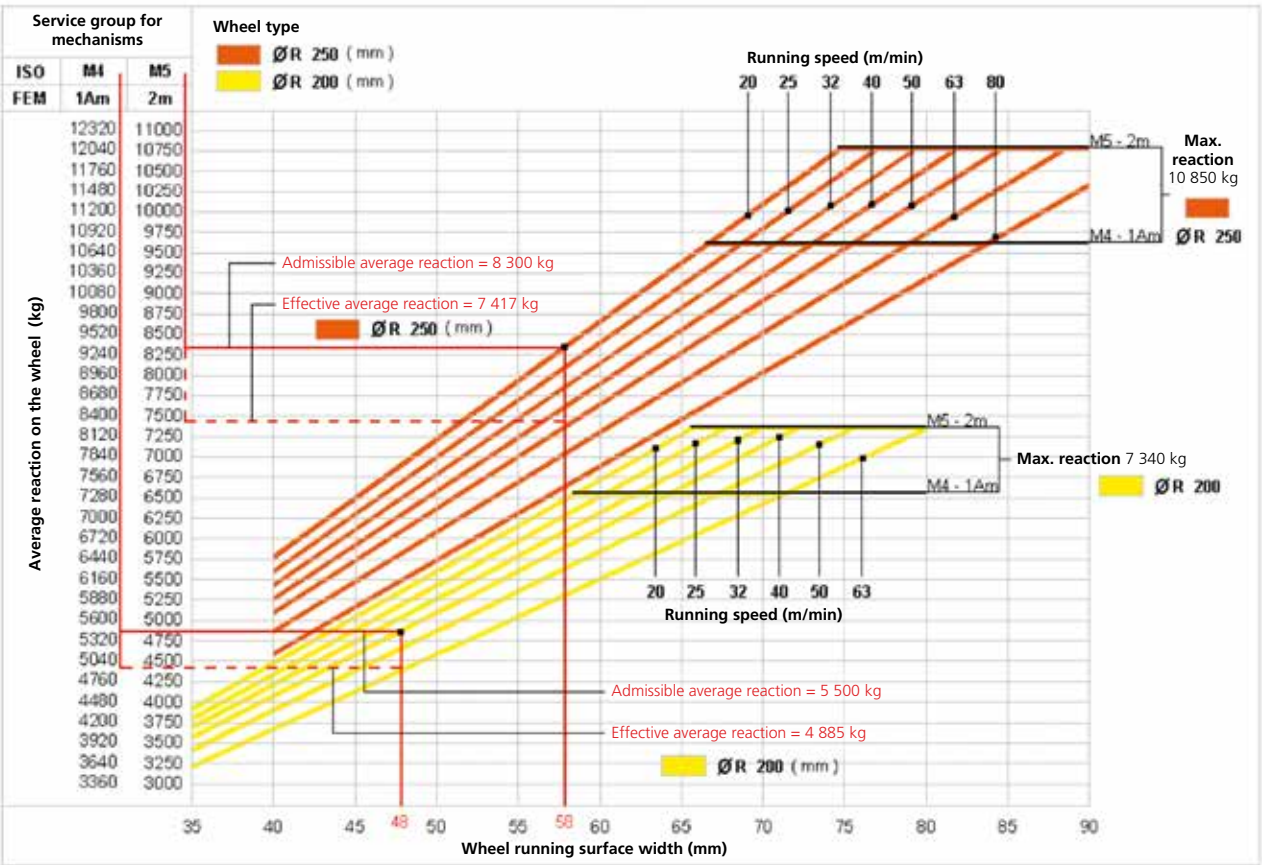
Example of verification of suitability for a Ø 200 wheel (see example 2 on page 26)
