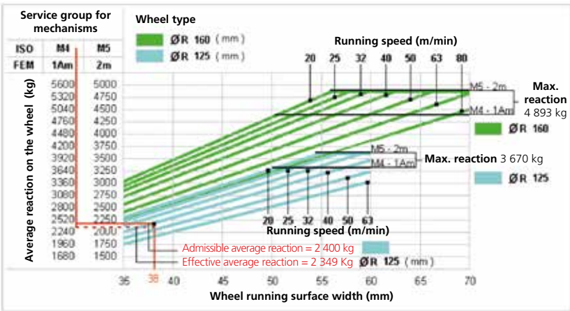
Example of verification of suitability for a Ø 125 wheel (see example 1 on page 36)
