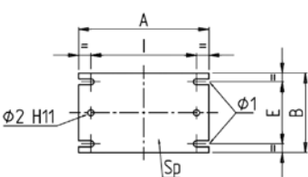
Connection plate for girder positioned laterally to the beam
